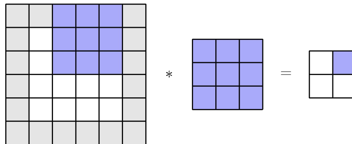
Strided convolution
