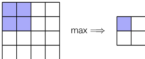
Max pooling
